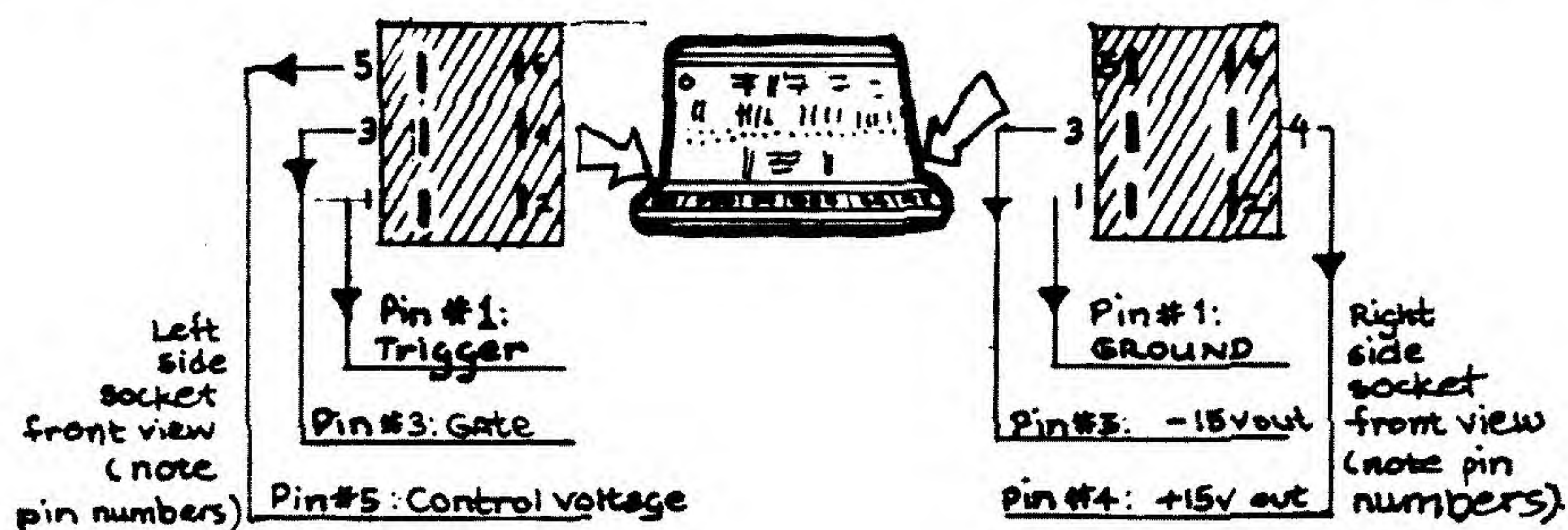
Power Connection
